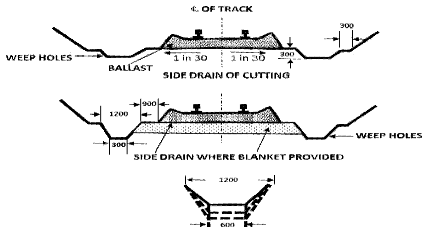
FIG. 5.4 DETAILS OF SIDE DRAINS
