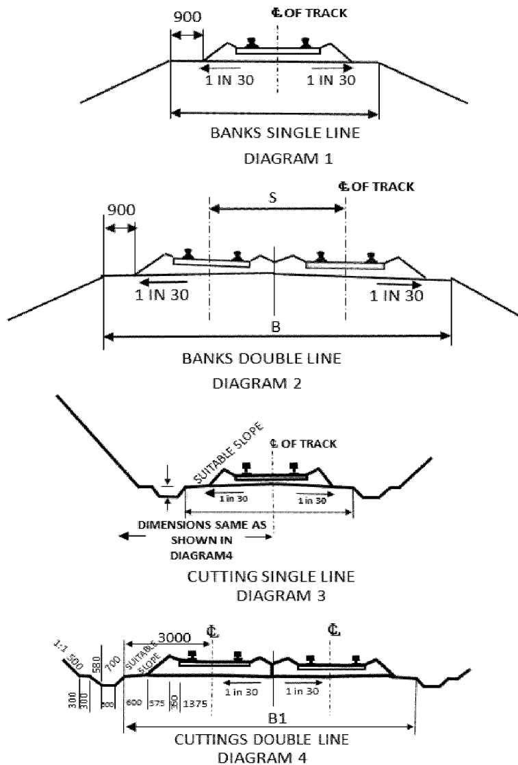
FIG. 5.3 MINIMUM/RECOMMENDED FORMATION WIDTHS FOR BANKS/CUTTINGS FOR CONCRETE SLEEPER TRACK
