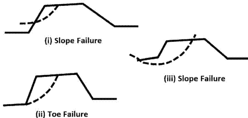
Fig 5.2 Types of Slope failure
