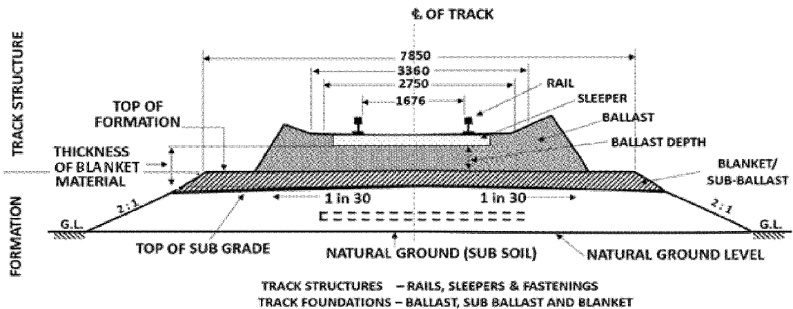
FIG. 5.1 FORMATION FOR BG TRACK
