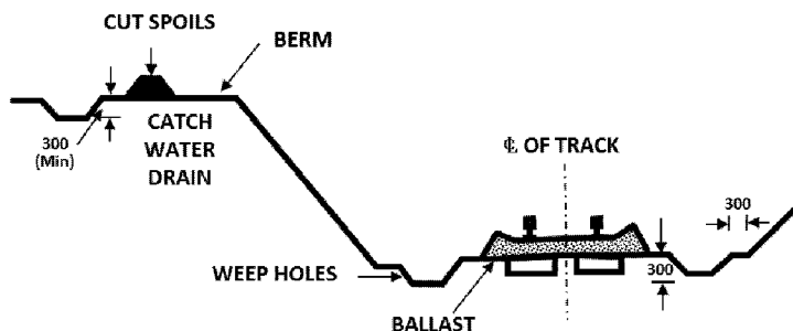
FIG. 5.5 DETAILS OF CATCH WATER DRAIN
